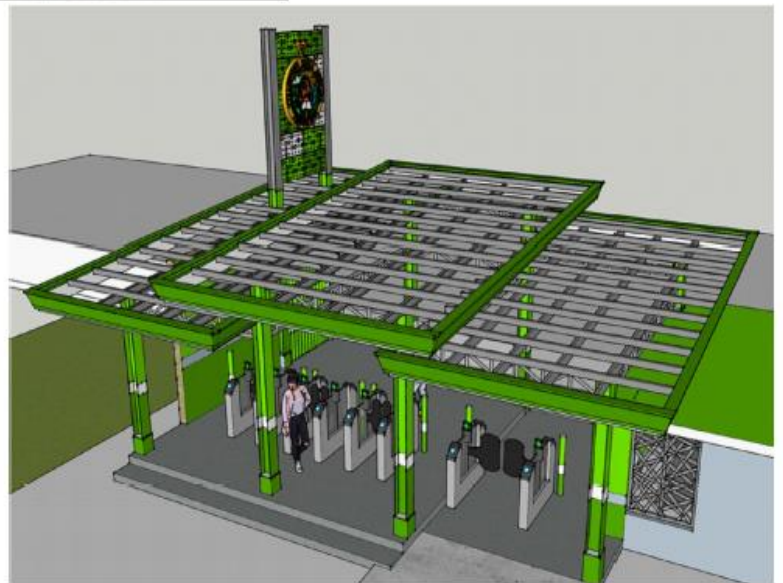
3D STRUCTURAL FRAME @ REAR SCALE: NTS
